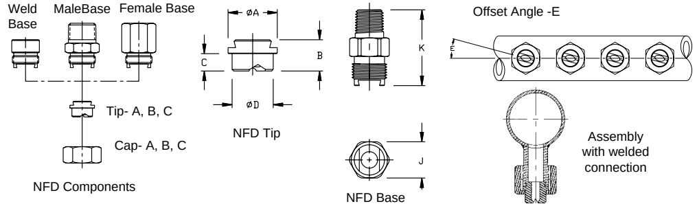
NFD Base
