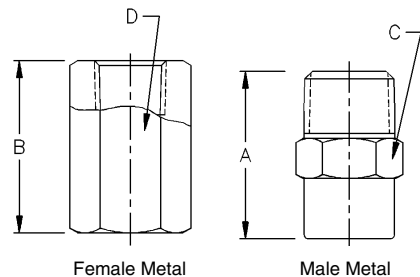
Female Metal
