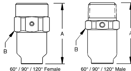
60° / 90° / 120° Female
