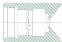
Carrier 10 (CI10) (shown) Carrier 12 (CI12) - without lugs
