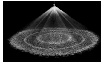
Full Cone 150°/170°
