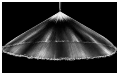
120° Hollow Cone
