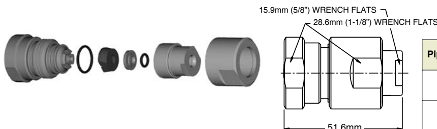
Female
